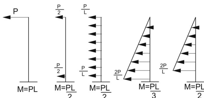
Figure 1 Bending Moments on an Unstayed Mast
