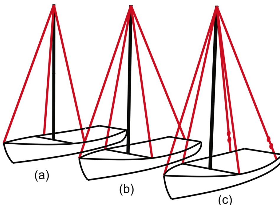
Figure 1: Staying Options for Single Panel Mast
