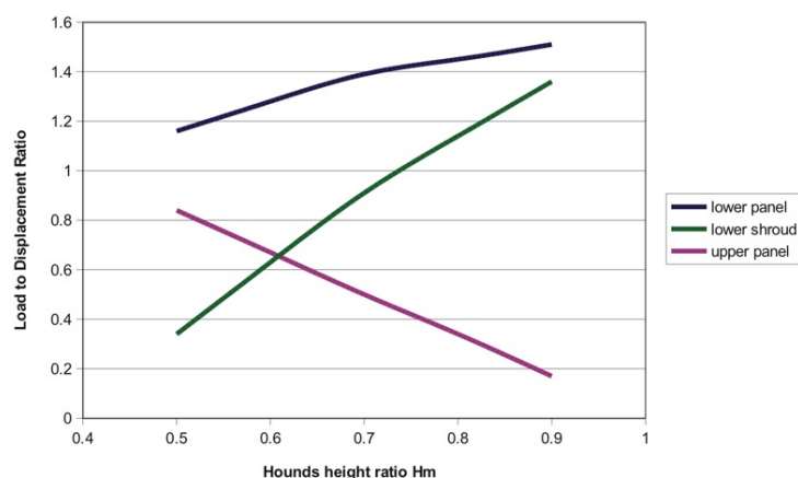
Figure 2: Effect on Lower Mast Load of Rig Height Sb 0.5, Hm 0.7
