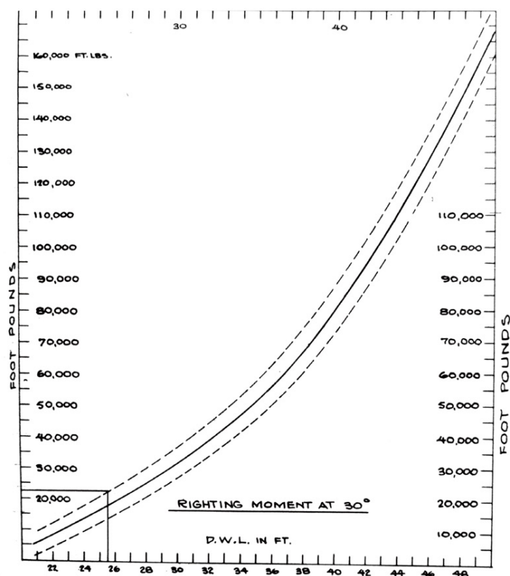
Figure 1: Righting Moment at 30° (From Kinney).
