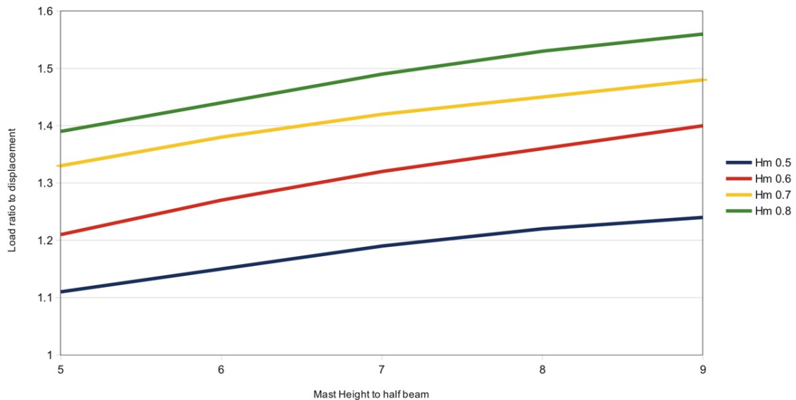
Figure 2: Lower Mast Design Load
