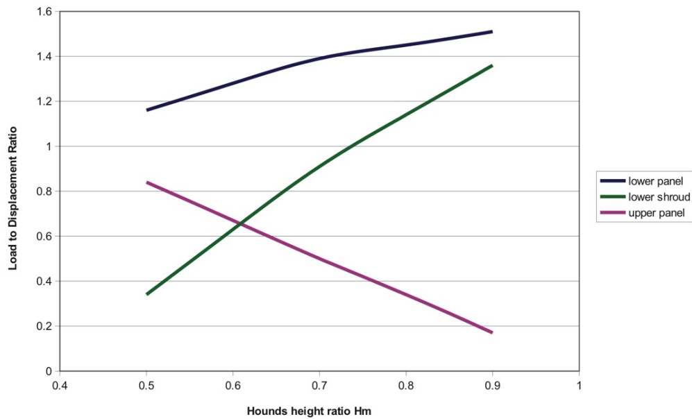
Figure 1: Effect on Lower Mast Load of Hounds Height
